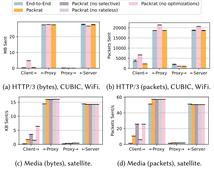
Fig. 9. Link Overhead. The number of bytes (left) and packets (right) sent between the client, proxy, and server. The link overheads from Packrat eACKs are comparable to those of the underlying acknowledgment scheme. Both clients send fewer bytes with rateless eACKs, and the media client sees fewer packets from selective eACKs (Section 5.2.2).
