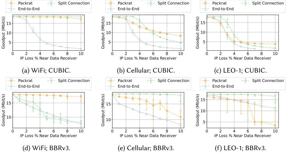
Fig. 5. Goodput of a large HTTP/3 file transfer using CUBIC and BBRv3 over the scenarios in Table 3 for a split, Packrat-assisted, and end-to-end connection. Packrat is able to recover in-network loss, outperforming end-to-end retransmissions when the latency between the client and proxy is relatively low, and typically approaching the goodput of a split connection.
