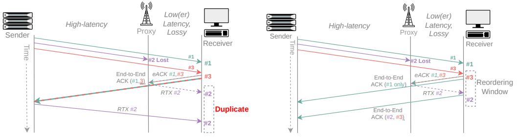
(a) Without selectively withheld acknowledgment gaps: the proxy retransmits packet #2, but it doesn't arrive before the receiver sends an end-to-end ACK that causes the sender to retransmit the same packet.
