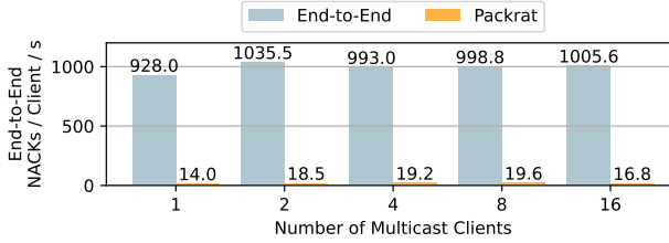
Fig. 7. Multicast benchmark over the cellular network setting (10% loss). Clients using Packrat send on average 59 \times fewer end-to-end NACKs than clients without Packrat. Other network scenarios see similar reductions in end-to-end retransmissions.
